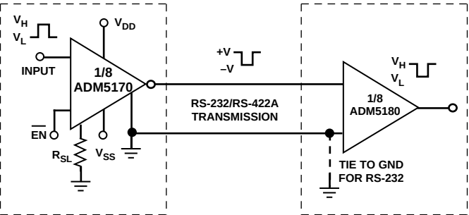
Figure 4. RS-232/RS-423A Typical Application Circuit
