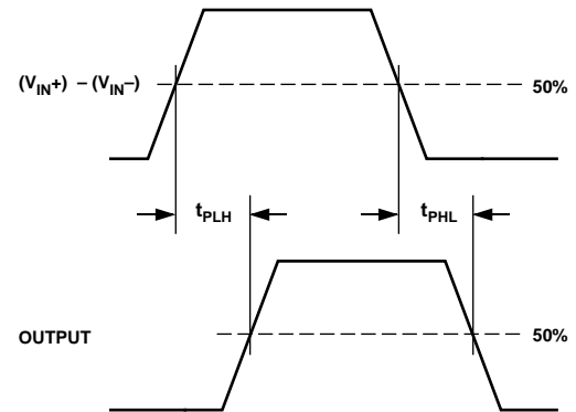
Figure 3. Timing Waveform
