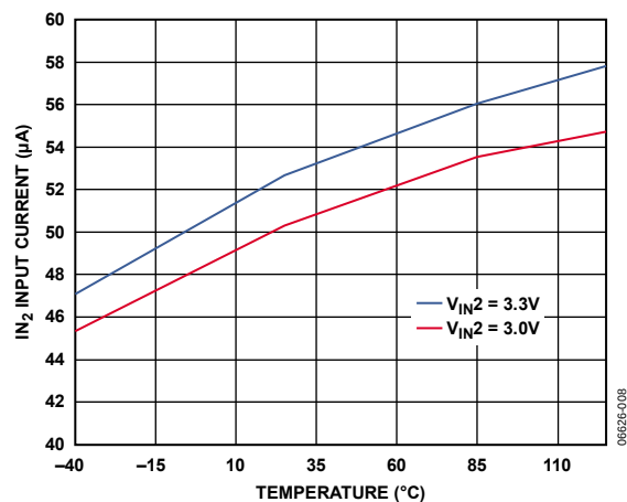
Figure 4. I_{IN2} Input Current vs. Temperature
