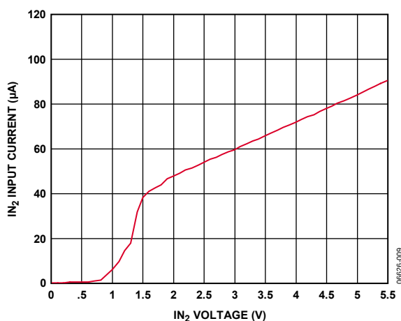
Figure 5. I_{IN2} Input Current vs. I_{IN2} Voltage
