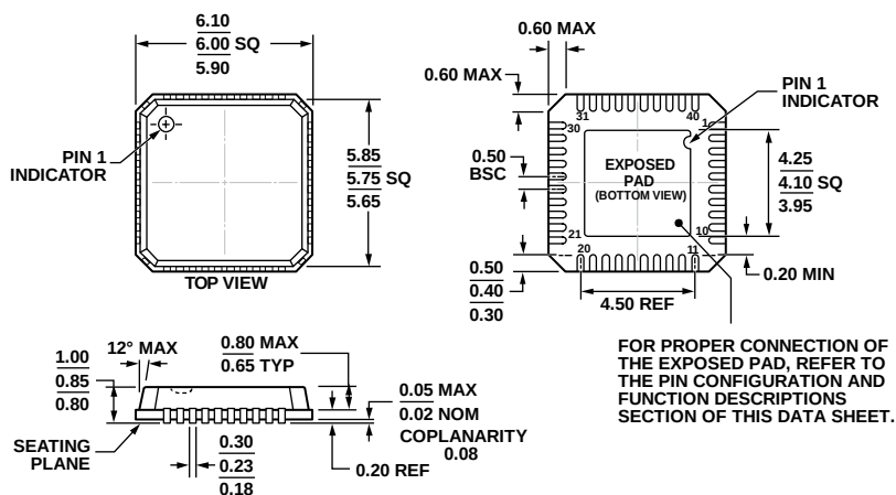
Figure 49. 40-Lead Lead Frame Chip Scale Package [LFCSP_VQ] 6 mm x 6 mm Body, Very Thin Quad (CP-40-1)
