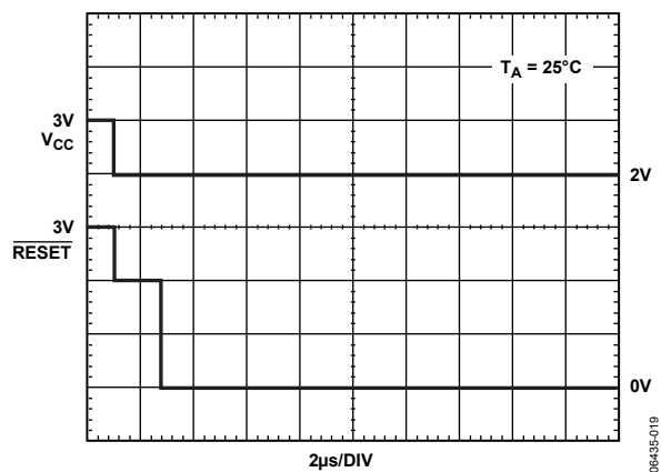
Figure 12. ADM706R/ADM706S/ADM706T and the ADM708R/ADM708S/ADM708T \overline{RESET} Response Time
