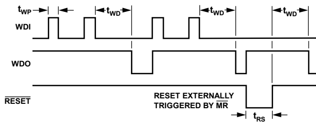
Figure 16. Watchdog Timing
