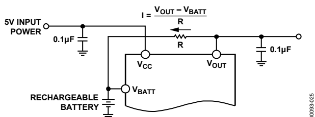
Figure 25. Rechargeable Battery
