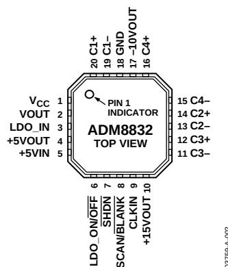
Figure 2. Pin Configuration
