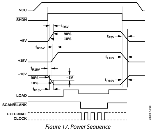
Figure 17. Power Sequence
