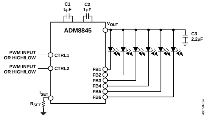
Figure 24. Digital PWM Brightness Control Application Diagram
