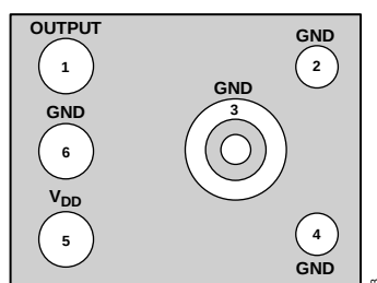
BOTTOM VIEW Not to Scale Figure 3. Pin Configuration (Bottom View)
