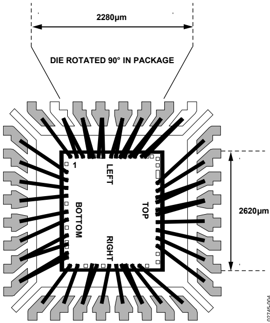
Figure 6. Bonding Diagram
