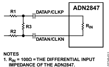
Figure 11. Attenuation Circuit
