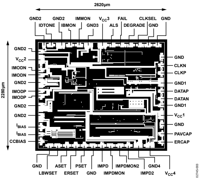
Figure 5. Metallization Photograph
