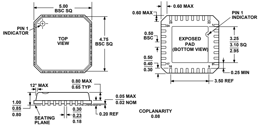
Figure 18. 32-Lead Lead Frame Chip Scale Package [LFCSP_VQ] 5 mm x 5 mm Body, Very Thin Quad (CP-32-2)
