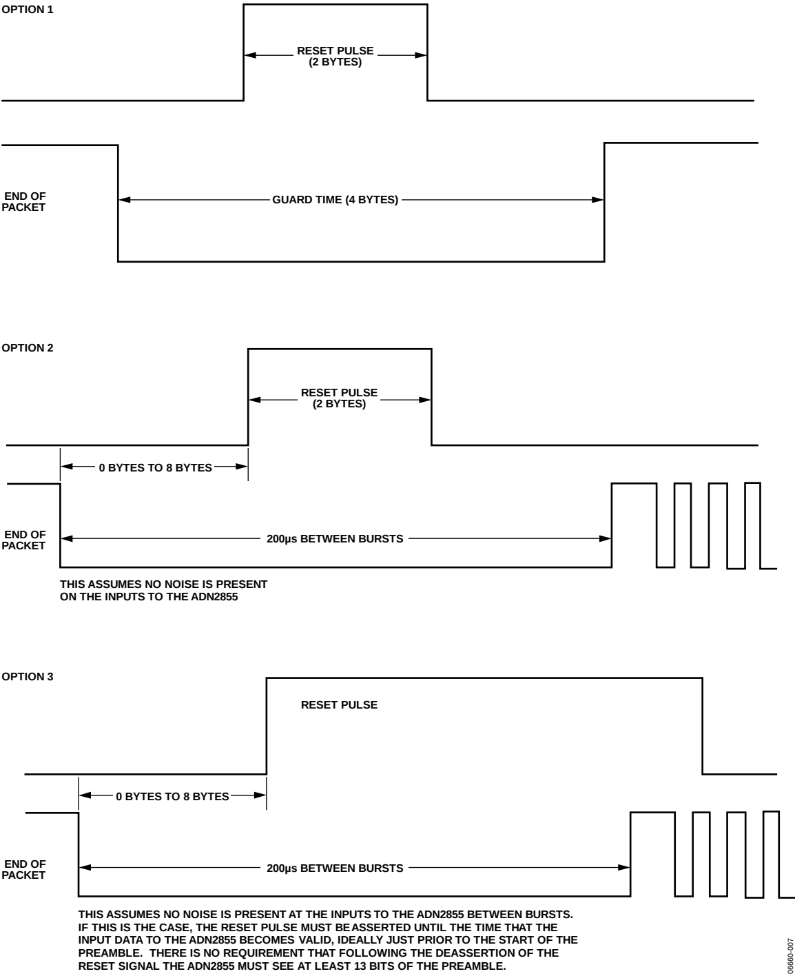
Figure 8. Reset Timing Options
