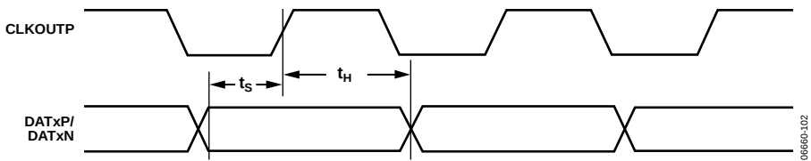
Figure 2. Output Timing
