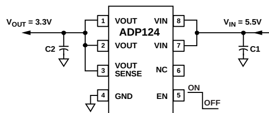
Figure 1. ADP124 with Fixed Output Voltage
