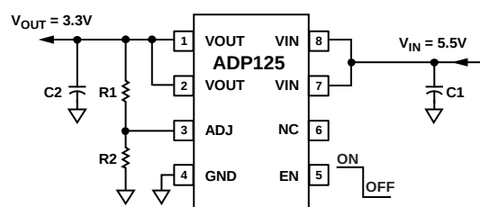
Figure 2. ADP125 with Adjustable Output Voltage
