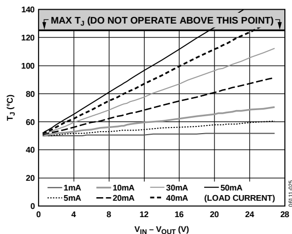
Figure 25. 300 \text{mm}^2 of PCB Copper, T_A = 50^{\circ}\text{C}
