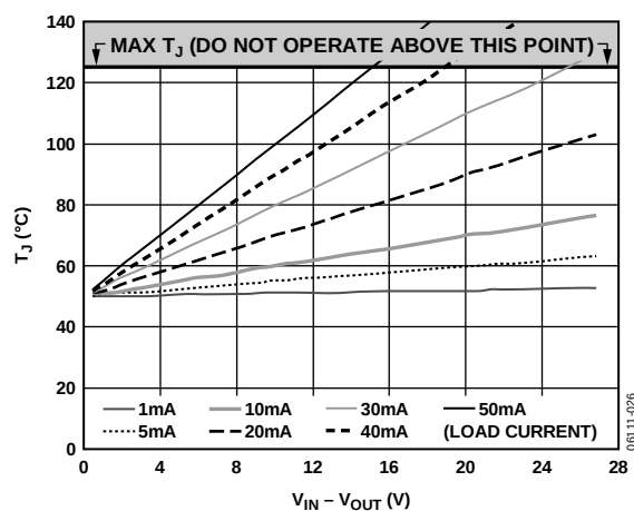
Figure 26. 100 \text{mm}^2 of PCB Copper, T_A = 50^{\circ}\text{C}
