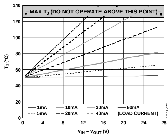
Figure 27. 0 \text{mm}^2 of PCB Copper, T_A = 50^{\circ}\text{C}
