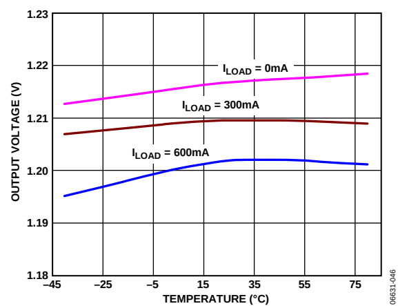
Figure 15. Output Voltage vs. Temperature ( V_{OUT} = 1.2\text{ V} )
