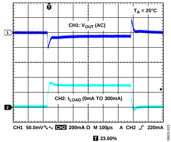
Figure 32. Load Transient Response ( V_{OUT} = 1.2\text{ V} )
