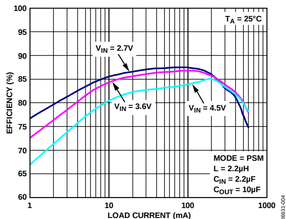
Figure 4. Efficiency vs. Load Current ( V_{OUT} = 1.2\text{ V} )
