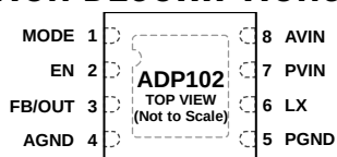
Figure 3. Pin Configuration
