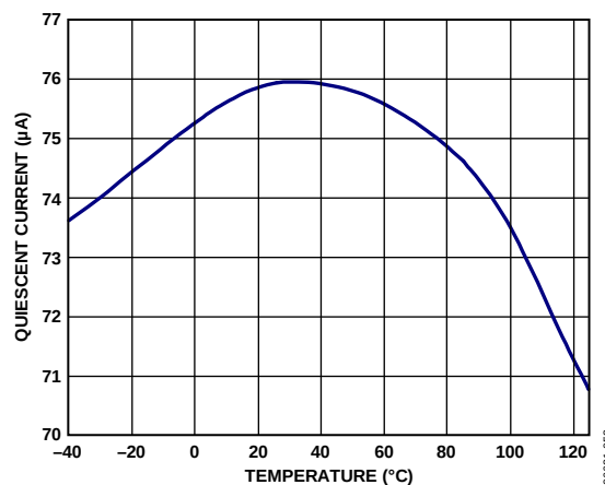
Figure 20. Quiescent Current vs. Temperature
