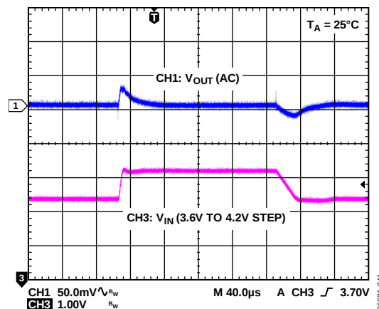
Figure 37. Line Transient Response ( V_{OUT} = 1.8\text{ V} )
