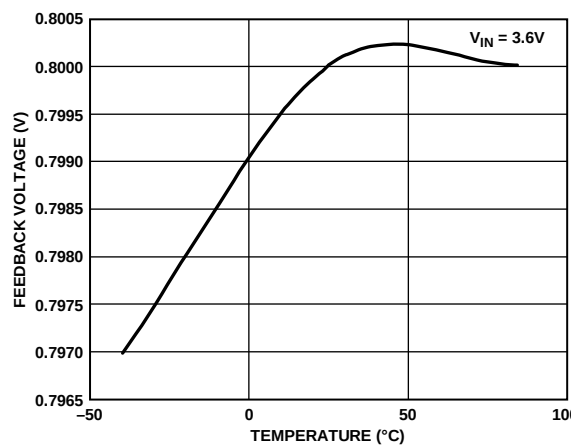
Figure 21. Feedback Voltage vs. Temperature
