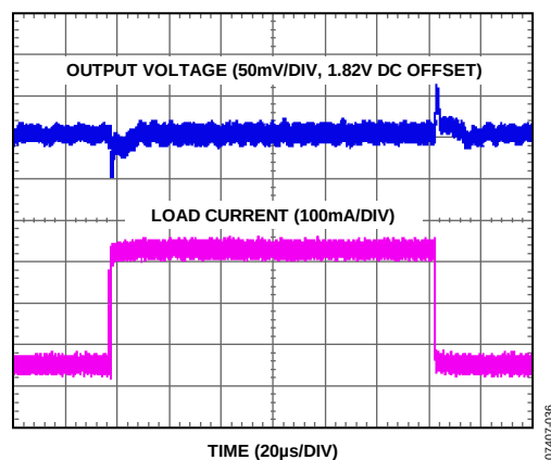
Figure 39. Load Transient Response, 150 mA to 400 mA ( V_{IN} = 4.5 V, PWM Mode)
