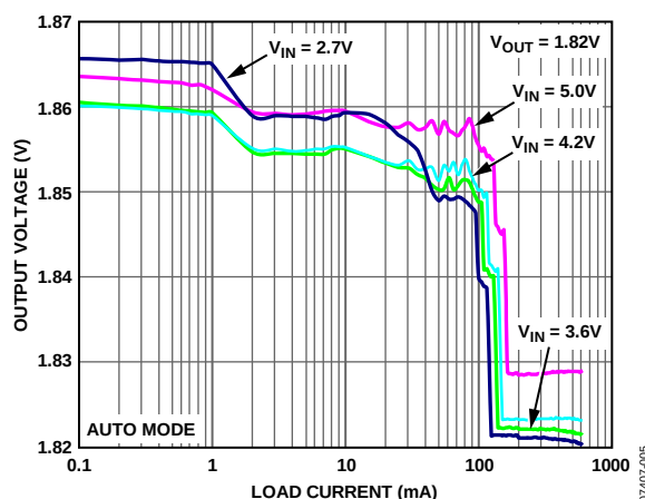
Figure 17. Output Voltage Accuracy (Auto Mode)
