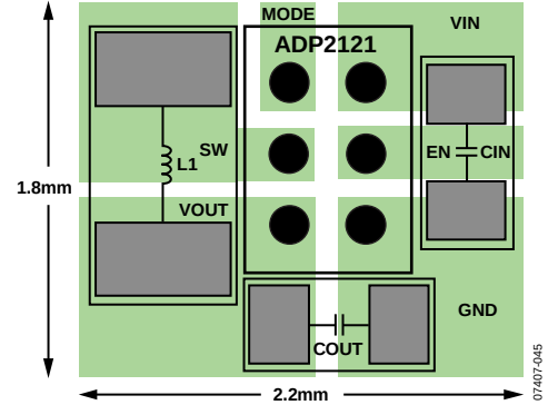
Figure 58. Solution Size with a 0603 Inductor
