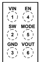
TOP VIEW (BALL SIDE DOWN) Not to Scale
