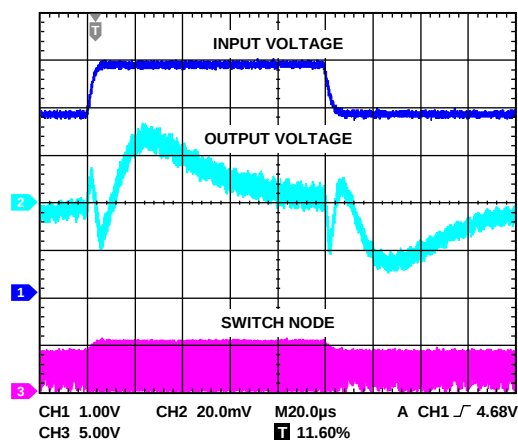
Figure 25. Line Transient, V_{OUT} = 3.3\text{ V} , PWM Mode, 600 mA, V_{IN1} = 4\text{ V} to 5 V, 4 \mu\text{s} Rise Time
