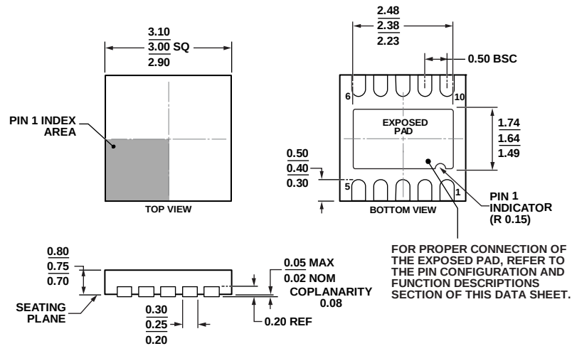
Figure 98. 10-Lead Lead Frame Chip Scale Package [LFCSP_WD] 3 mm × 3 mm Body, Very Very Thin, Dual Lead (CP-10-9) Dimensions shown in millimeters
