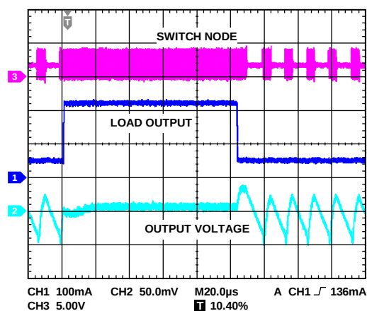
Figure 27. Load Transient, V_{OUT} = 1.8\text{ V} , 50 mA to 250 mA, Load Current Rise Time = 200 ns
