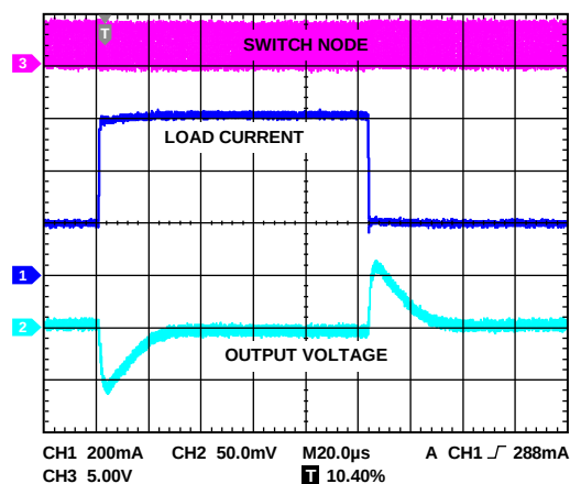
Figure 26. Load Transient, V_{OUT} = 1.8\text{ V} , 200 mA to 600 mA, Load Current Rise Time = 200 ns
