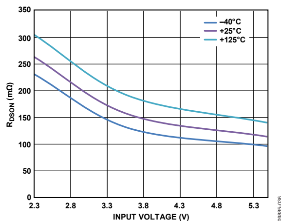
Figure 12. R_{DS(on)} PFET vs. Input Voltage, Across Temperature
