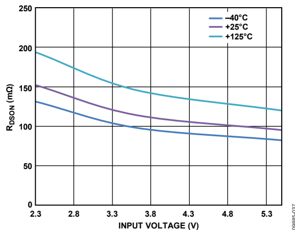
Figure 13. R_{DS(on)} NFET vs. Input Voltage, Across Temperature
