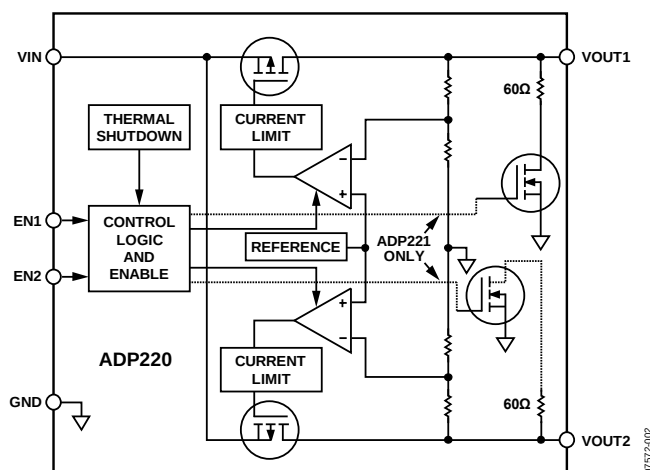
Figure 2. Block Diagram of the ADP220/ADP221
