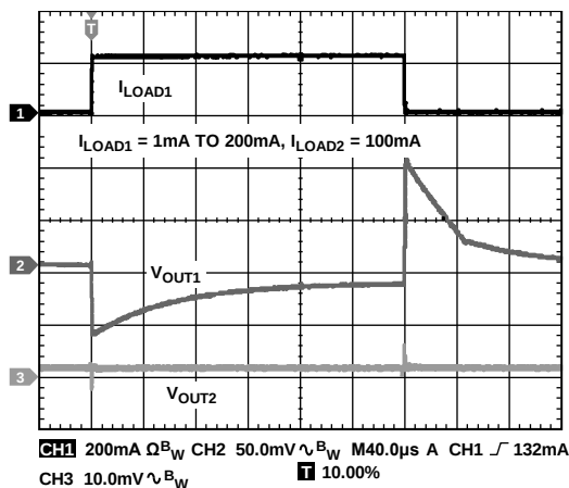
Figure 24. Load Transient Response, I_{LOAD1} = 1mA to 200mA , I_{LOAD2} = 100mA , CH1 = I_{LOAD1} , CH2 = V_{OUT1} , CH3 = V_{OUT2}
