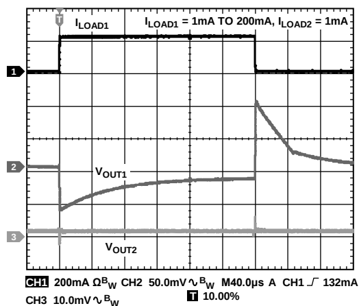
Figure 23. Load Transient Response, I_{LOAD1} = 1mA to 200mA , I_{LOAD2} = 1mA CH1 = I_{LOAD1} , CH2 = V_{OUT1} , CH3 = V_{OUT2}
