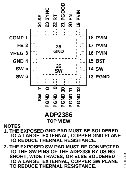
Figure 3. Pin Configuration
