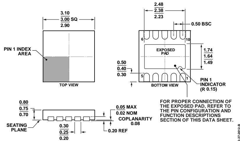
Figure 32. 10-Lead Lead Frame Chip Scale Package [LFCSP_WD] 3 mm x 3 mm Body, Very Very Thin, Dual Lead (CP-10-9)
