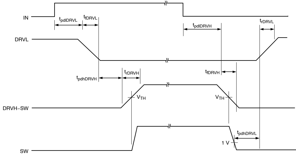
Figure 4. Timing Diagram
