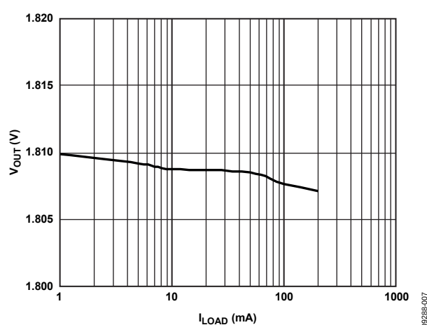
Figure 9. Output Voltage vs. Load Current, V_{RIPPLE} = 50\text{ mV} , C_{OUT} = 1\text{ }\mu\text{F}
