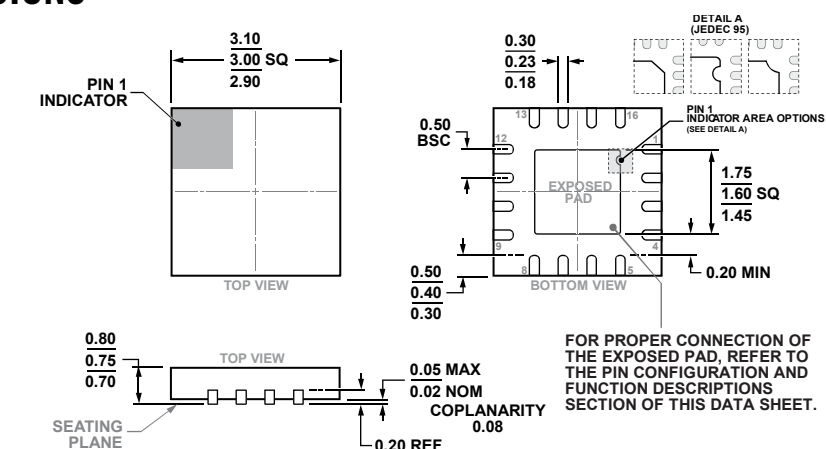
Figure 64. 16-Lead Lead Frame Chip Scale Package [LFCSP] 3 mm x 3 mm Body and 0.75 mm Package Height (CP-16-22) Dimensions shown in millimeters
