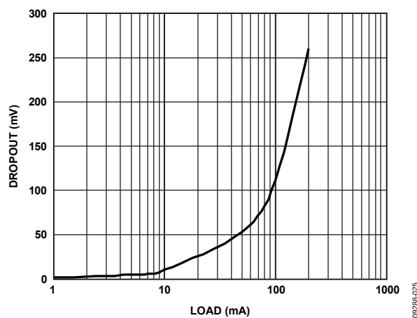
Figure 27. Dropout Voltage vs. Load Current and Output Voltage, V_{OUT2} = 1.8 \text{ V} , V_{RIPPLE} = 50 \text{ mV} , C_{OUT} = 1 \mu\text{F}
