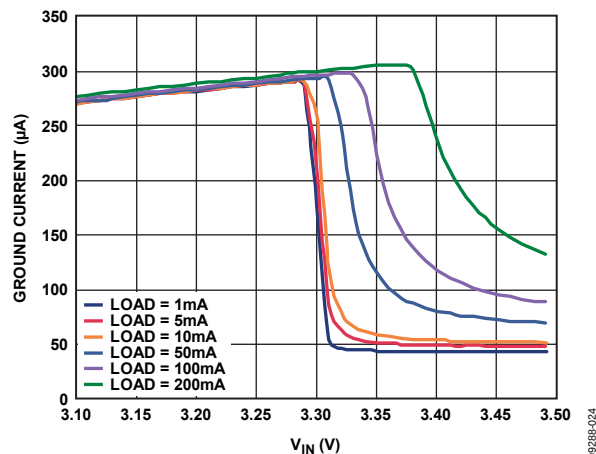
Figure 26. Ground Current vs. Input Voltage (in Dropout), V_{OUT1} = 3.3 \text{ V} , V_{RIPPLE} = 50 \text{ mV} , C_{OUT} = 1 \mu\text{F}
