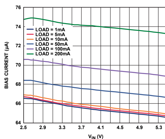
Figure 22. Bias Current vs. Input Voltage, Single Output Loaded, V_{RIPPLE} = 50\text{ mV} , C_{OUT} = 1\text{ }\mu\text{F}
