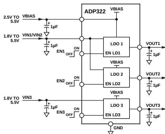
Figure 1. Typical Application Circuit for ADP322
