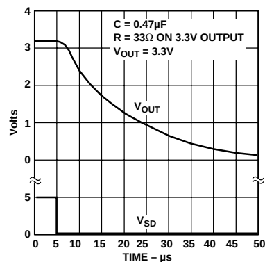
Figure 17. Turn-Off
