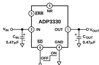
Figure 1. Typical Application Circuit
