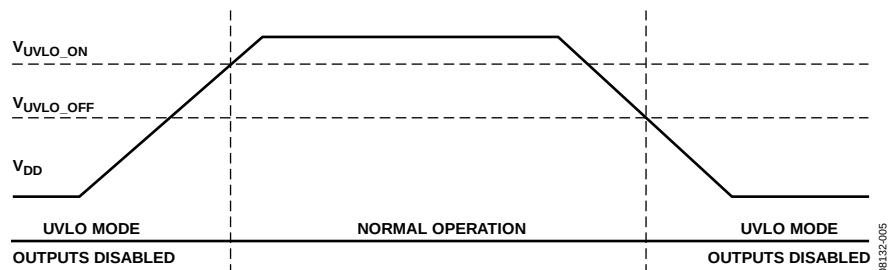
Figure 5. UVLO Function
