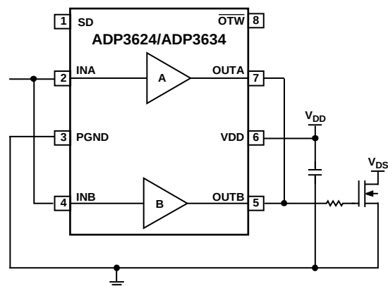
Figure 25. Parallel Operation
