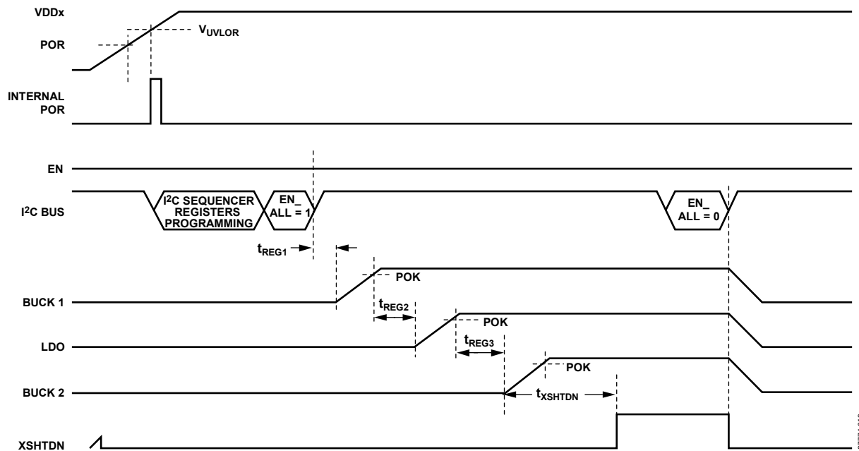
Figure 23. Regulators Are Activated by I²C Command
