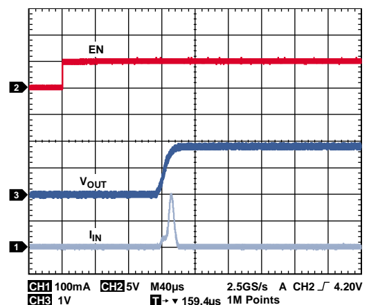
Figure 30. LDO Startup, V_{OUT3} = 1.8 V
