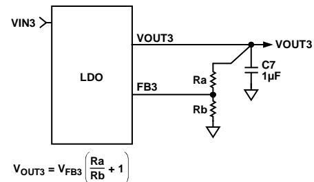
Figure 48. LDO External Output Voltage Setting
