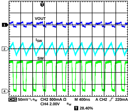
Figure 21. Typical Waveforms, V_{OUT1} = 3.3\text{ V} , I_{OUT1} = 30\text{ mA} , PWM Mode
