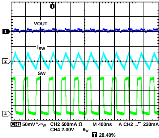
Figure 22. Typical Waveforms, V_{OUT2} = 1.8\text{ V} , I_{OUT2} = 30\text{ mA} , PWM Mode
