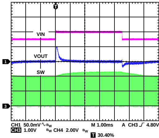
Figure 23. BUCK1 Response to Line Transient, Input Voltage from 4.5\text{ V} to 5.0\text{ V} , V_{OUT1} = 3.3\text{ V} , PWM Mode
