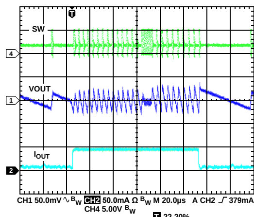
Figure 26. BUCK2 Response to Load Transient, I_{OUT2} from 1\text{ mA} to 50\text{ mA} , V_{OUT2} = 1.8\text{ V} , Auto Mode
