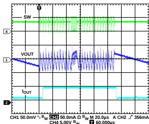
Figure 25. BUCK1 Response to Load Transient, I_{OUT1} from 1\text{ mA} to 50\text{ mA} , V_{OUT1} = 3.3\text{ V} , Auto Mode
