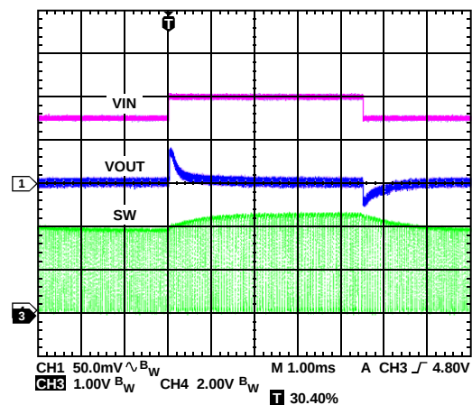
Figure 24. BUCK2 Response to Line Transient, V_{IN2} = 4.5\text{ V} to 5.0\text{ V} , V_{OUT2} = 1.8\text{ V} , PWM Mode
