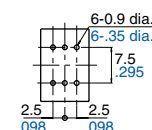
Recommended PC board pattern (TOP VIEW 2:1)
