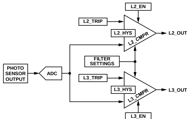
Figure 31. Ambient Light Sensing and Trip Comparators
