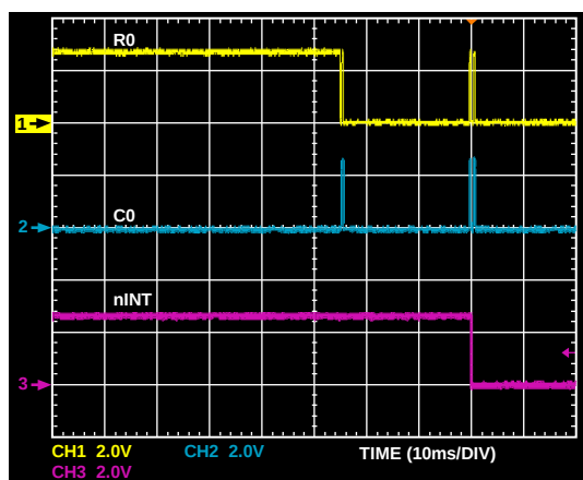
Figure 36. Key Press(R0,C0)
