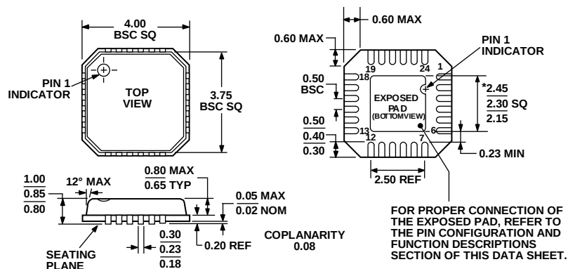
Figure 61. 24-Lead Lead Frame Chip Scale Package [LFCSP_VQ] 4 mm x 4 mm Body, Very Thin Quad (CP-24-2) Dimensions shown in millimeters
