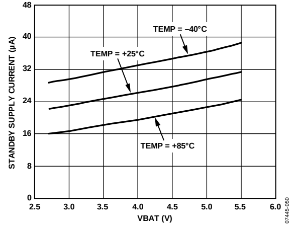
Figure 7. Standby Supply Current vs. V BAT
