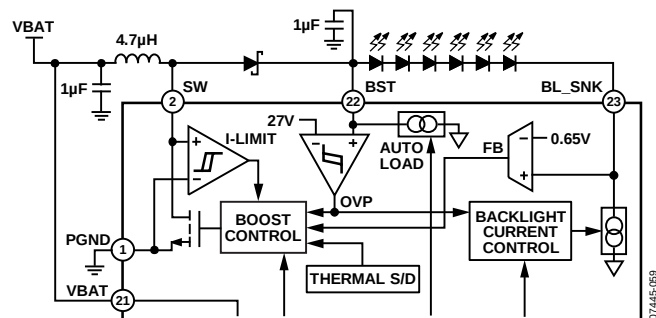
Figure 51. Boost Configuration
