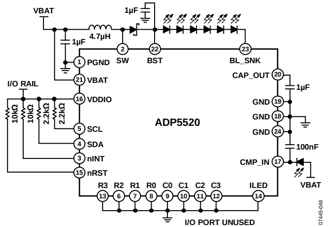
Figure 60. I/O Configuration Example 8
