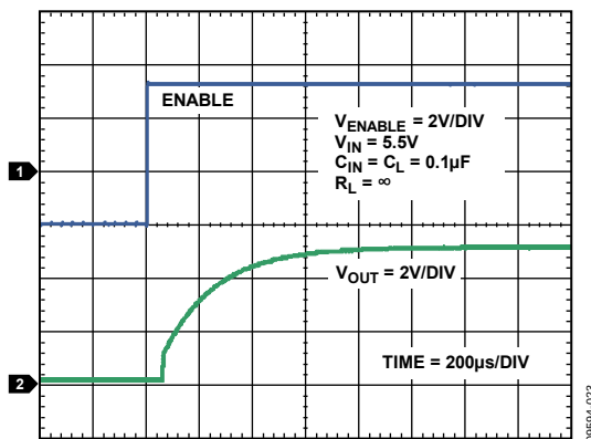
Figure 23. ADR3550 Restart Response from Shutdown
