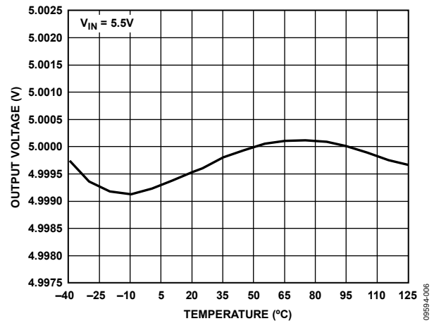
Figure 6. ADR3550 Output Voltage vs. Temperature
