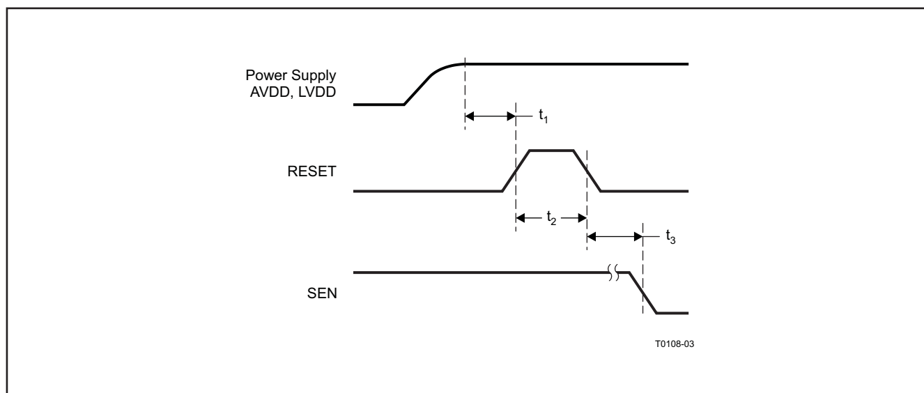
Figure 5. Reset Timing
