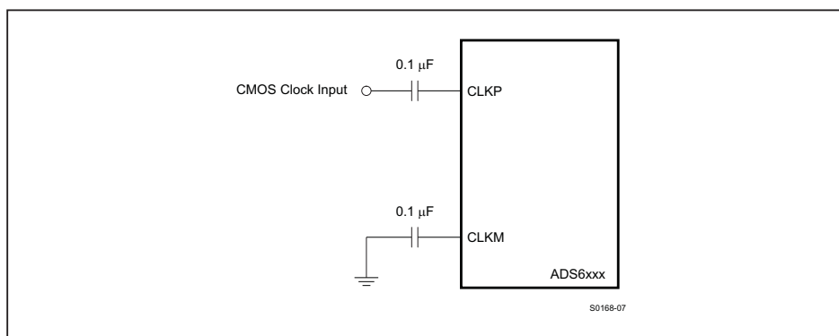
Figure 92. Single-Ended Clock Driving Circuit
