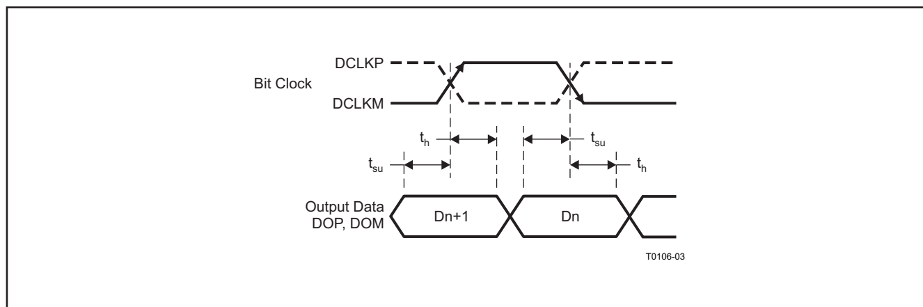
Figure 2. LVDS Timings
