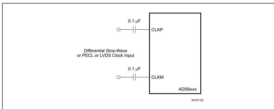
Figure 90. Differential Clock Driving Circuit
