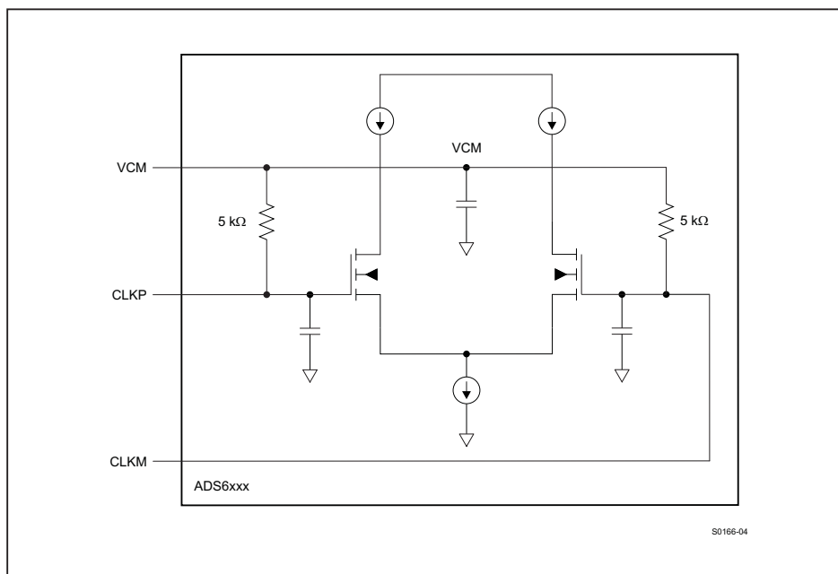
Figure 89. Internal Clock Buffer
