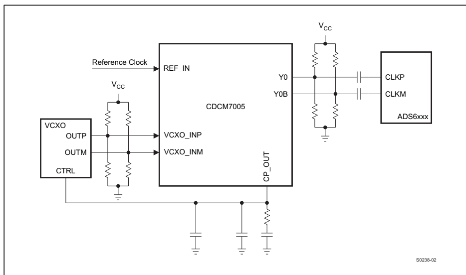
Figure 91. PECL Clock Drive Using CDCM7005
