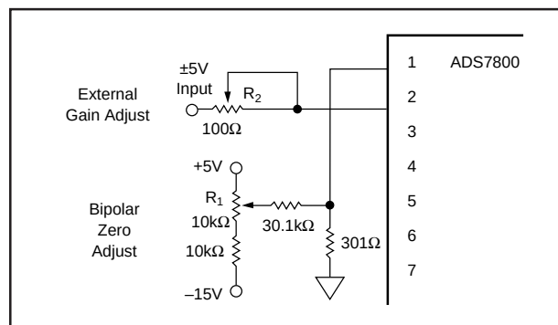
FIGURE 11. \pm 5 V Range With External Trims.
