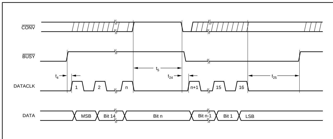
FIGURE 8. Serial Data Timing, External Clock, Clocking After the Conversion Completes and During the Next Conversion (EXT/INT HIGH, \overline{\text{CS}} LOW).
