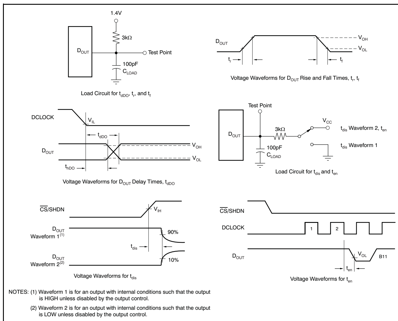
Figure 23. Timing Diagrams and Test Circuits for the Parameters in Table 1
