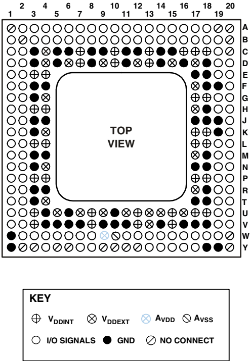
Figure 50. 256-Ball BGA_ED Ball Configuration (Top View)
