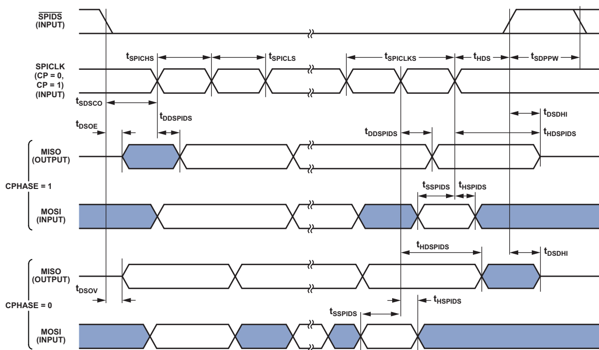
Figure 37. SPI Slave Timing
