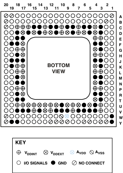
Figure 49. 256-Ball BGA_ED Ball Configuration (Bottom View)
