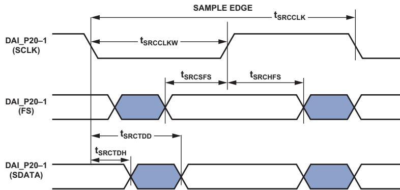
Figure 30. SRC Serial Output Port Timing
