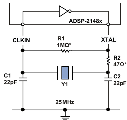
Figure 7. Recommended Circuit for Fundamental Mode Crystal Operation
