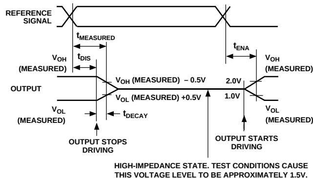
Figure 12. Output Enable/Disable
