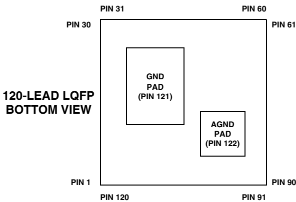
Figure 90. 120-Lead LQFP Package Lead Configuration (Bottom View)
