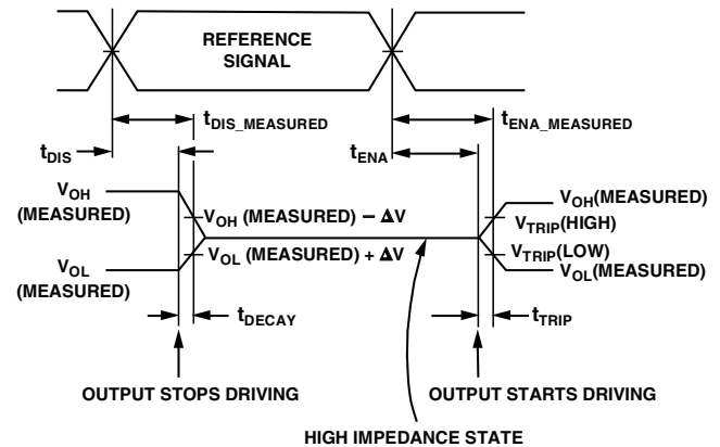
Figure 42. Output Enable/Disable
