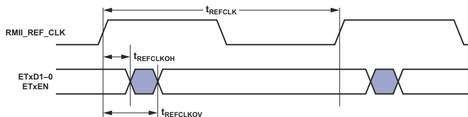
Figure 36. 10/100 Ethernet MAC Controller Timing: RMII Transmit Signal
