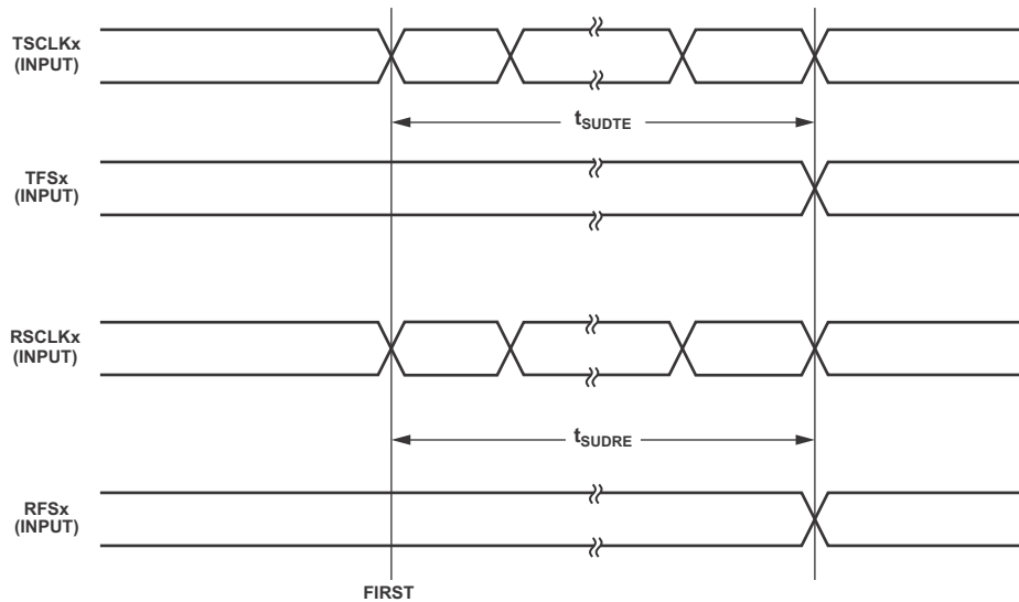
Figure 24. Serial Port Start Up with External Clock and Frame Sync
