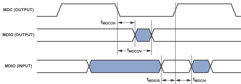
Figure 38. 10/100 Ethernet MAC Controller Timing: MII Station Management
