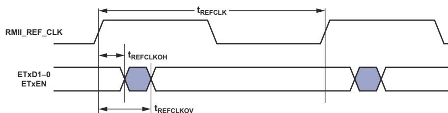
Figure 36. 10/100 Ethernet MAC Controller Timing: RMIIT Transmit Signal
