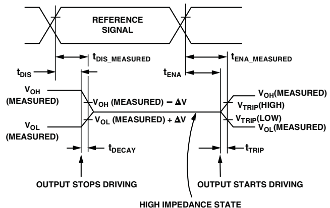
Figure 73. Output Enable/Disable
