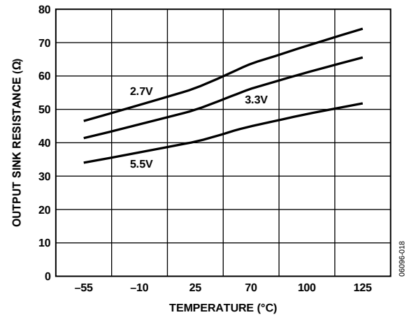
Figure 8. Output Sink Resistance vs. Temperature
