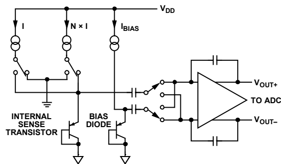
Figure 44. Top Level Structure of Internal Temperature Sensors
