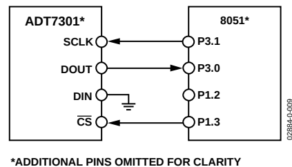
Figure 16. ADT7301-to-8051 Interface
