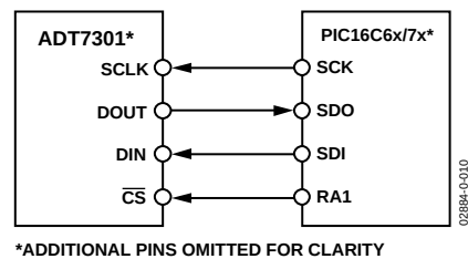
Figure 17. ADT7301-to-PIC16C6x/7x Interface
