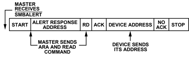
Figure 59. INT/ \overline{\text{INT}} Responds to \overline{\text{SMBALERT}} ARA
