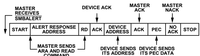
Figure 60. INT/ \overline{\text{INT}} Responds to \overline{\text{SMBALERT}} ARA with Packet Error Checking (PEC)
