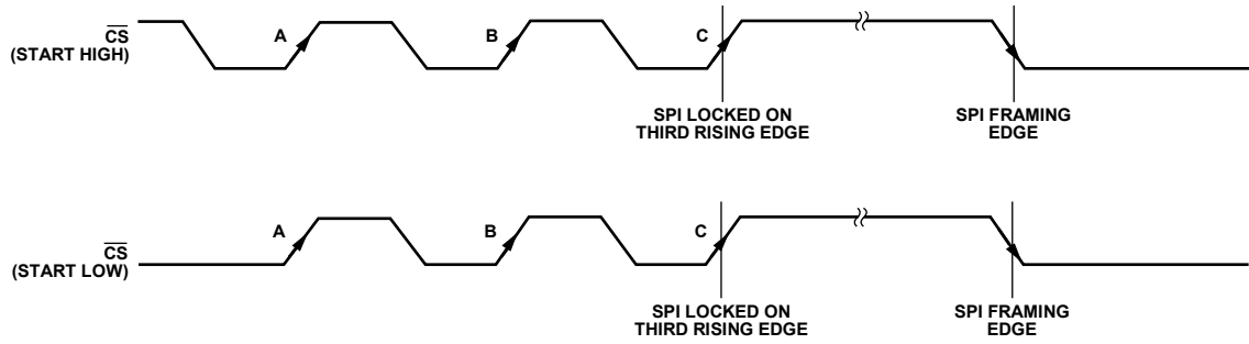
Figure 50. Serial Interface—Selecting and Locking SPI Protocol
